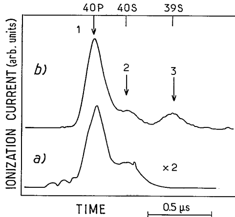
FIG. 3. Time-resolved atomic ionization signals (trace a) below threshold and (trace b) above threshold for two-photon maser emission. The arrows indicate the times at which levels 40P , 40S , and 39S ionize in the electric field ramp. Appearance of peak 3 in trace (b) is evidence for maser action. Detection sensitivity is twice as large in trace (a) as in trace (b).
